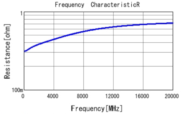
GRM0225C1E1R7CA03 R DCOV, 25degC
