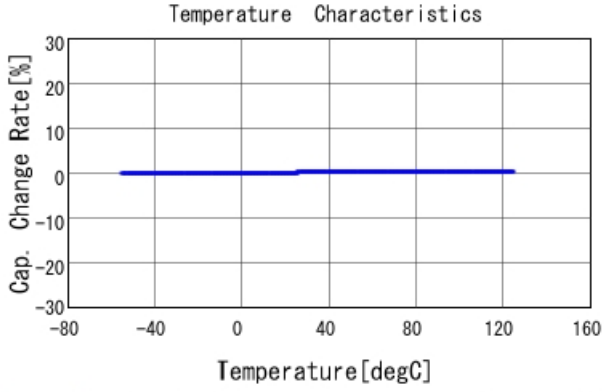
GRM0225C1E1R7CA03 C-Temp. capchange, DCOV, AC1Vrms
