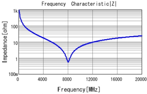
GRM0225C1E1R7CA03 |Z| DCOV, 25degC
