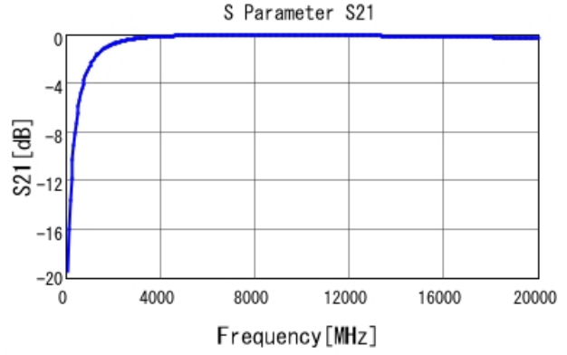
GRM0225C1E1R7CA03 S21 DCOV, 25degC
