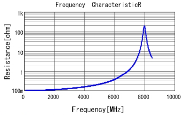
GQM1875C2E5R0BB12 R DCOV, 25degC
