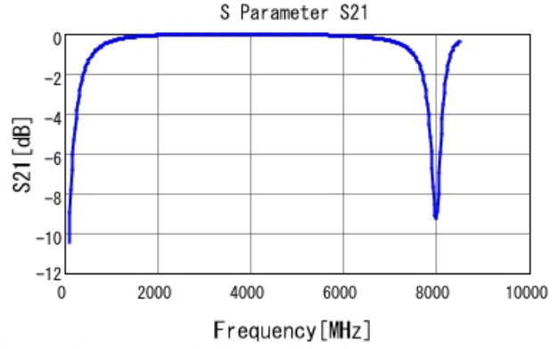
GQM1875C2E5R0BB12 S21 DC0V, 25degC
