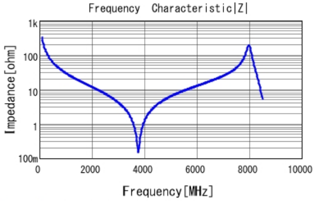
GQM1875C2E5R0BB12 |Z| DCOV, 25degC
