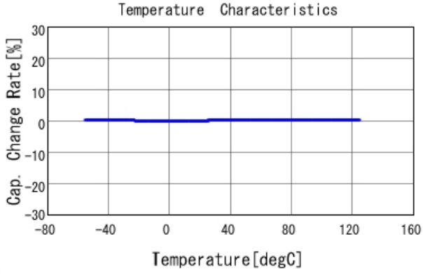
GQM1875C2E5R0BB12 C-Temp. capchange, DC0V, AC1Vrms
