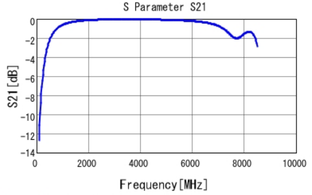
GRM1885C2A3R8CA01 S21 DCOV, 25degC
