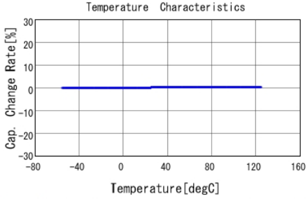
GRM1885C2A3R8CA01 C-Temp. capchange, DCOV, AC1Vrms
