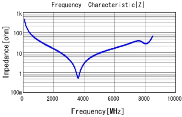
GRM1885C2A3R8CA01 |Z| DCOV, 25degC
