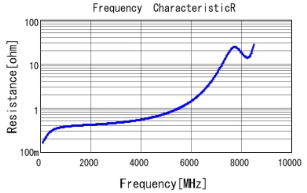
GRM1885C2A3R8CA01 R DCOV, 25degC
