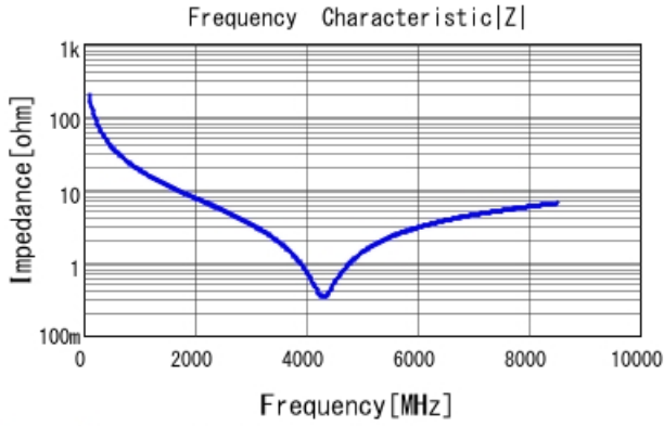
GRM0225C1E8R1CA03 |Z| DCOV, 25degC
