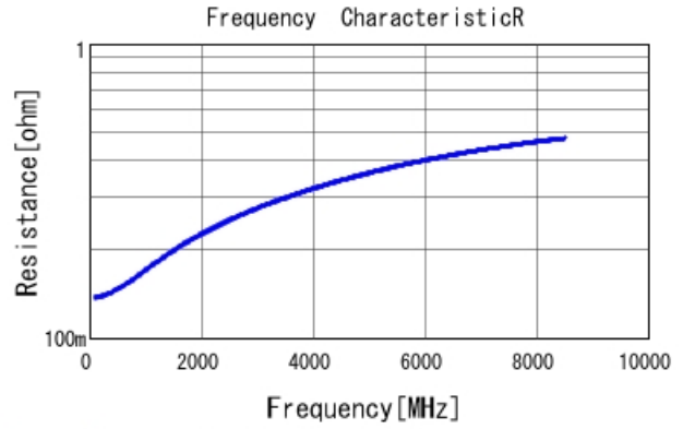
GRM0225C1E8R1CA03 R DCOV, 25degC
