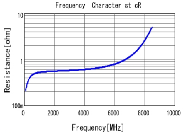
■ GRM1885C2A1R9CA01 R DC0V, 25degC
