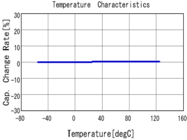
■ GRM1885C2A1R9CA01 C-Temp. capchange, DCOV, AC1Vrms
