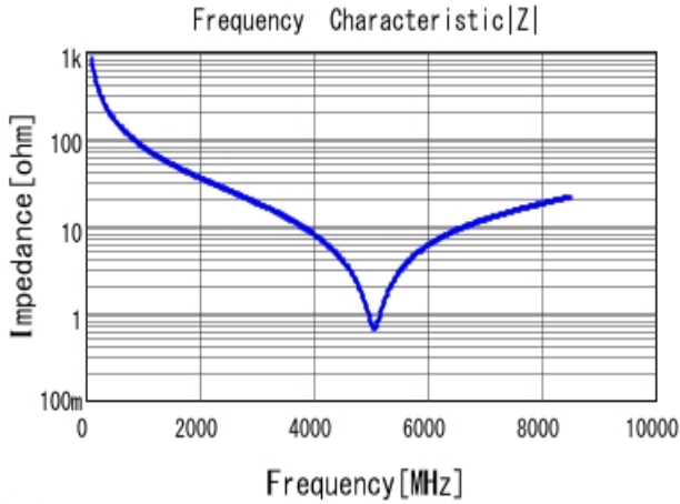
■ GRM1885C2A1R9CA01 |Z| DC0V, 25degC
