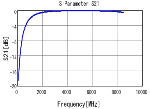
■ GRM1885C2A1R9CA01 S21 DCOV, 25degC
