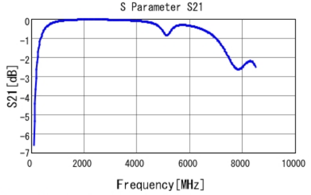
GRM1885C1H8R4DA01 S21 DCOV, 25degC
