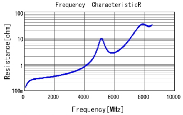
GRM1885C1H8R4DA01 R DCOV, 25degC
