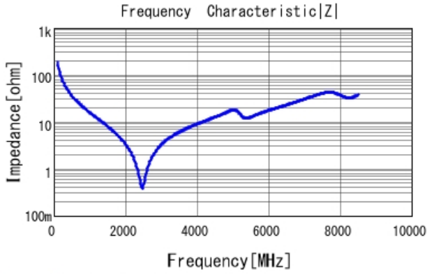
GRM1885C1H8R4DA01 |Z| DCOV, 25degC
