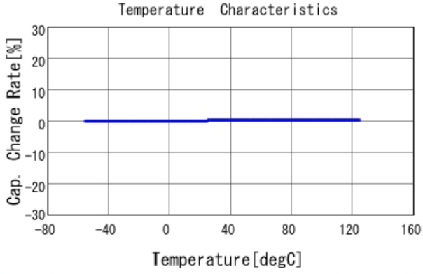
GRM1885C1H8R4DA01 C-Temp. capchange, DCOV, AC1Vrms
