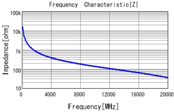
GJM1555C1HR10WB01 |Z| DCOV, 25degC
