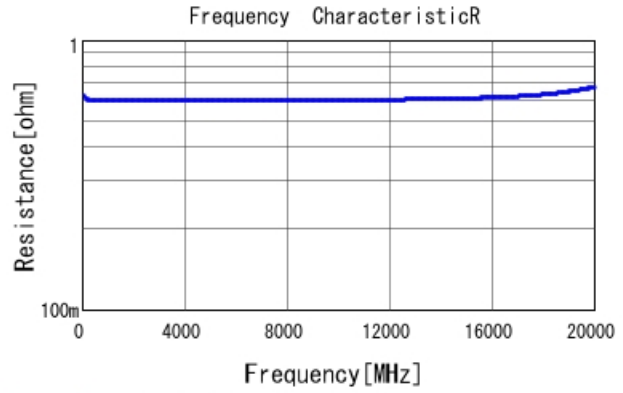
GJM1555C1HR10WB01 R DCOV, 25degC
