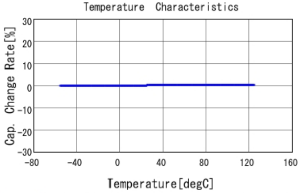
GRM1885C1H1R2BA01 C-Temp. capchange, DCOV, AC1Vrms
