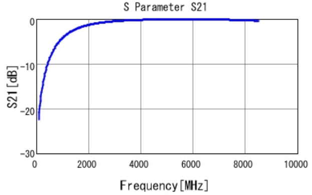
GRM1885C1H1R2BA01 S21 DCOV, 25degC
