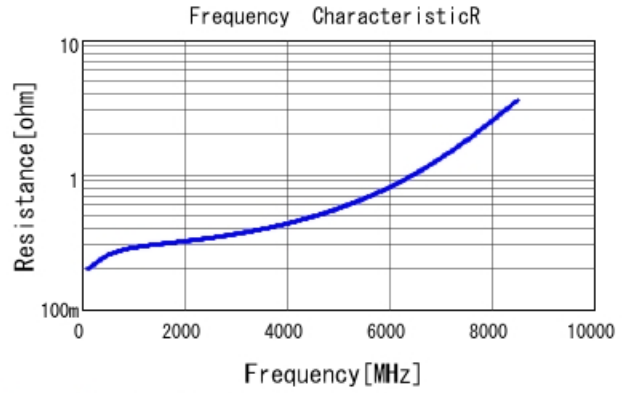
GRM1885C1H1R2BA01 R DCOV, 25degC
