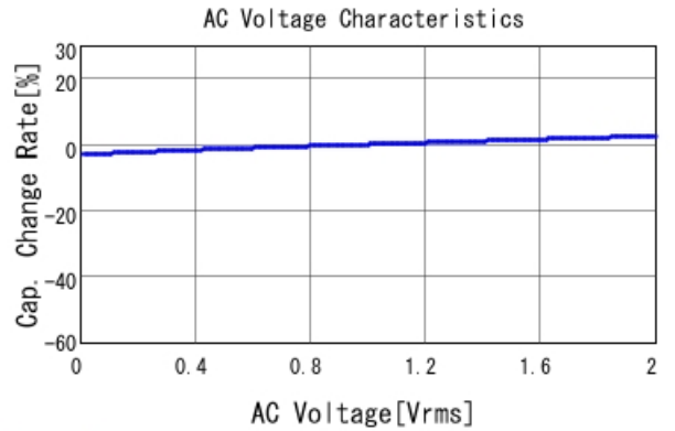
GCJ31CR72A105KA01 C-AC Voltage capchange, DC0V, 25
