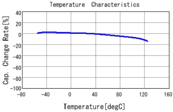
GCJ31CR72A105KA01 C-Temp. capchange, DC0.0V, AC1.C
