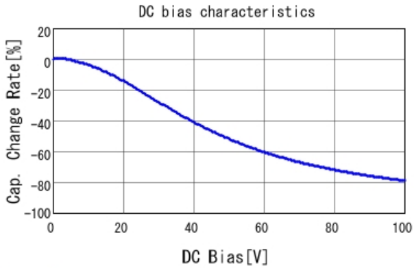
GCJ31CR72A105KA01 C-DC bias capchange, 25.0degC, A
