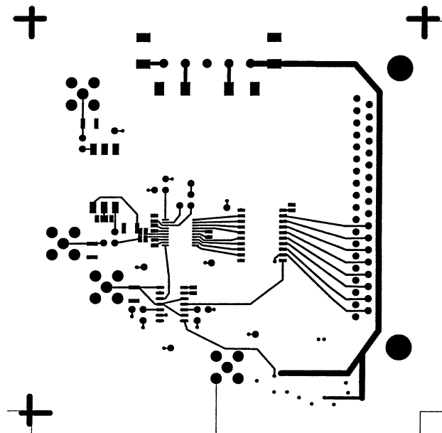
Figure 9. Printed Circuit Board Top Side Copper
