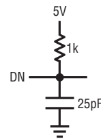
(B) V_{OL} TO Hi-Z
