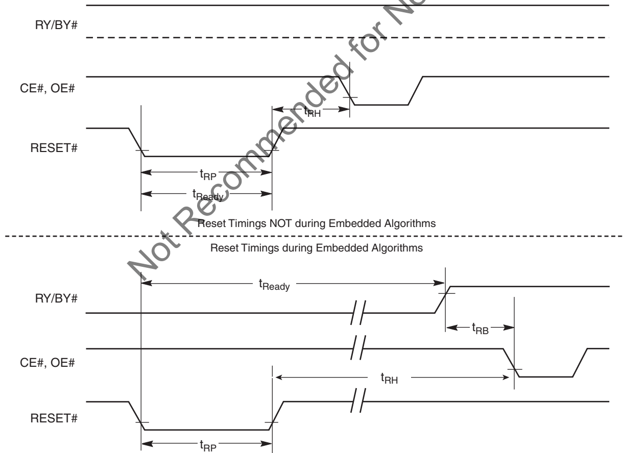
Figure 17.2 RESET# Timings
