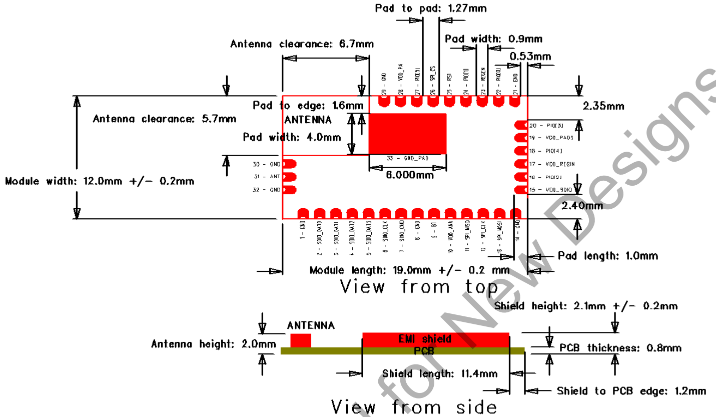
Figure 9.1. Physical Dimensions
