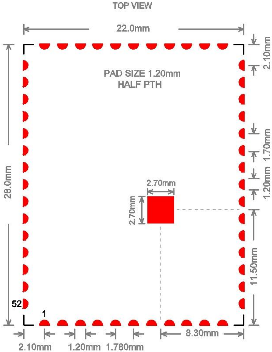
Figure 3: Package Dimensions
