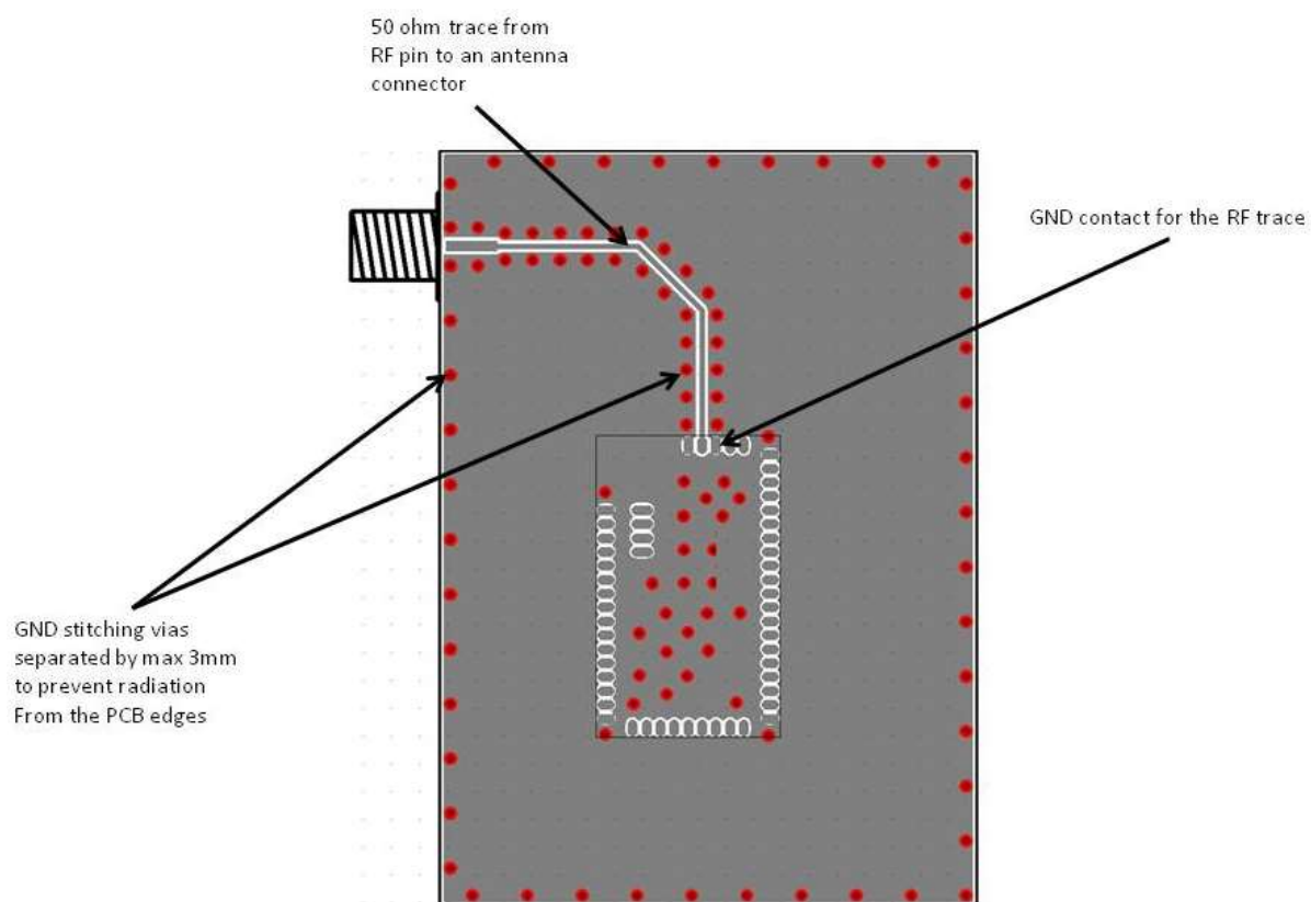
Figure 6: Typical 50 ohm trace from the RF pin to an antenna connector
