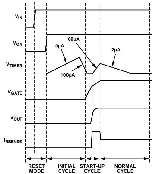
Figure 31. Power-Up into Capacitor
