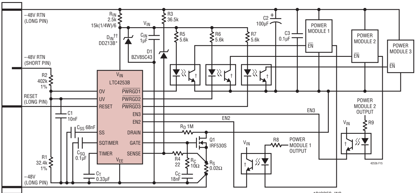
Figure 15. Power Limit Circuit Breaker Application
