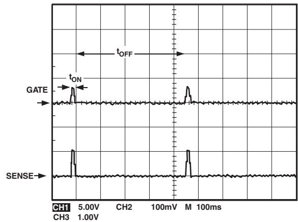
Figure 11. Illustration of the PWM Ratio ( t_{ON}/t_{OFF} )
