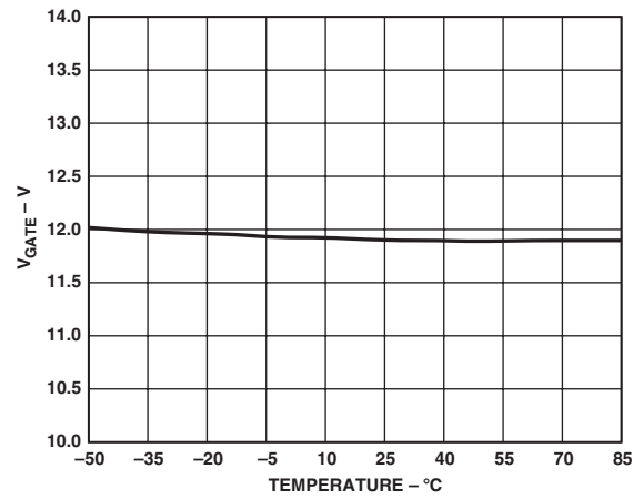
TPC 11. V_{GATE} vs. Temperature
