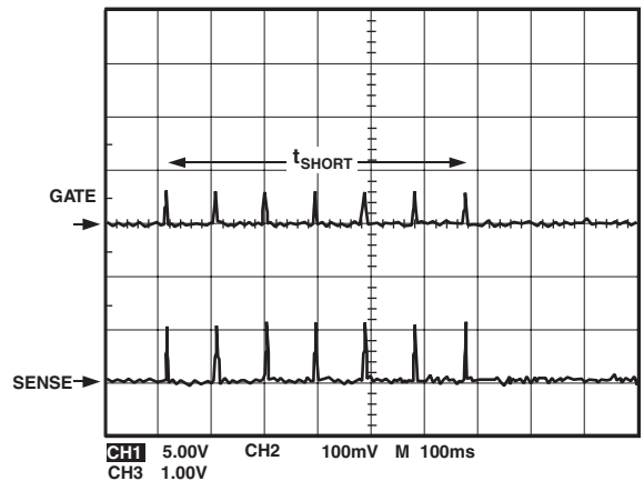
Figure 12. Illustration of the Limited Consecutive Retry Function (Seven Retries and Latch Off)
