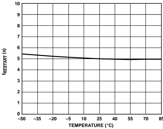
Figure 28. t_{RESTART} Time vs. Temperature
