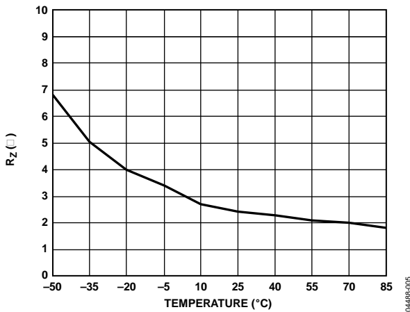
Figure 5. R Z (V IN Forward Voltage) vs. Temperature
