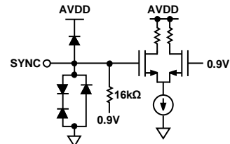
Figure 25. Equivalent SYNC Input Circuit
