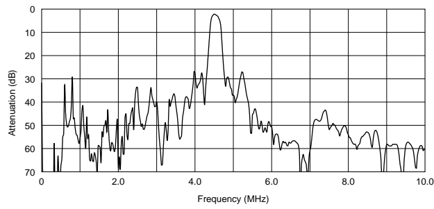
SFSKA6M00CF00-R1
