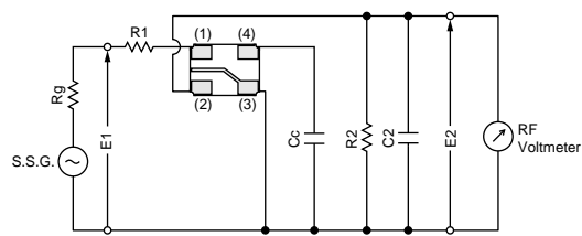
SFSKB2M30GF00-R1/SFSKB3M20GF00-R1
