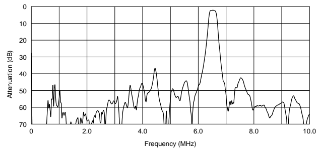
SFSKA6M50CF00-R1
