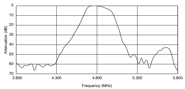
SFSKB4M80GF00-R1
