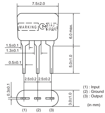
SFELG10M7KA00-B0
