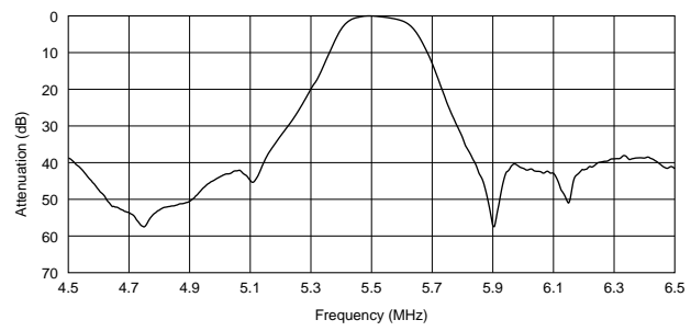
SFSKA5M50CF00-R1
