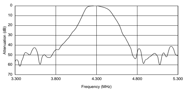
SFSKB4M30GF00-R1
