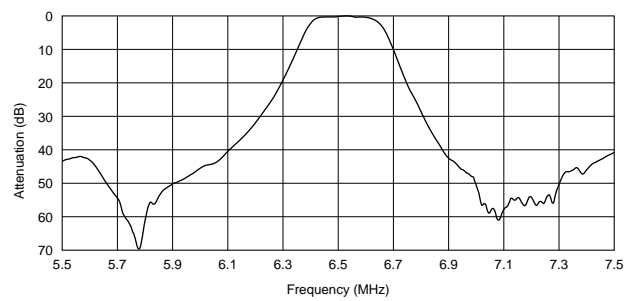
SFSKA6M50CF00-R1
