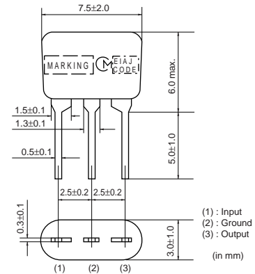
SFELG10M7HA00-B0
