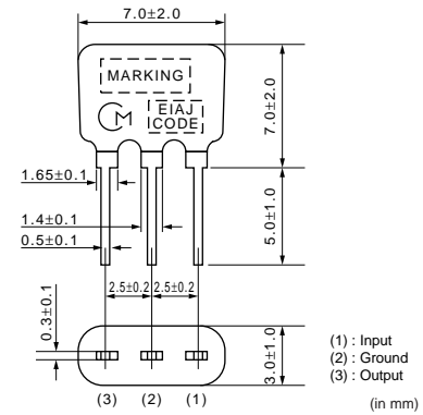
SFVLF10M7MF00-B0
