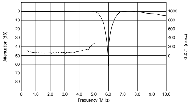
TPSKA6M00B00-R1
