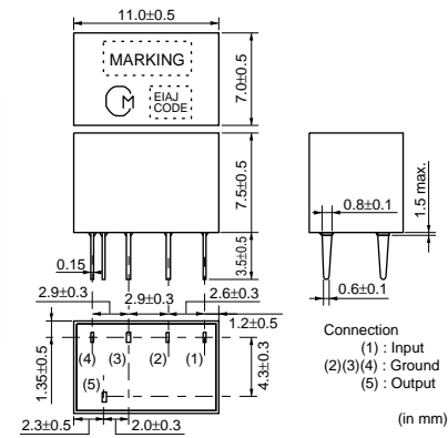
CFWLA Series
