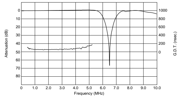
TPSKA6M50B00-R1
