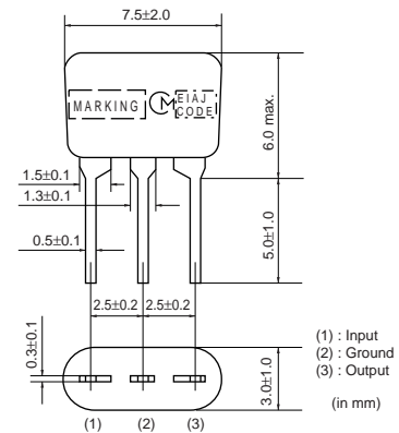
SFELG10M7FA00-B0
