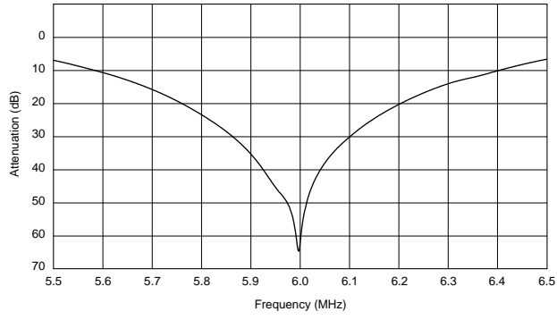
TPSKA6M00B00-R1
