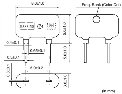
CDALF10M7C_Series
