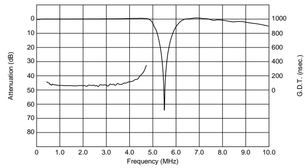
TPSKA5M50B00-R1
