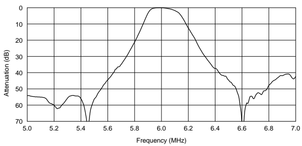
SFSKA6M00CF00-R1
