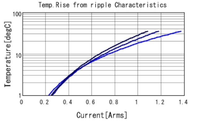
GRM1555C2A101GA01 Temp. rise — 200MHz — 500I
