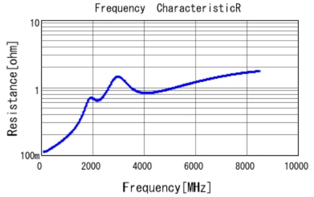
GRM1555C2A101GA01 R DCOV, 25degC
