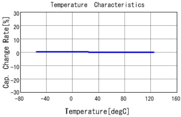
GRM1555C2A101GA01 C-Temp. capchange, DCOV, AC1Vrms
