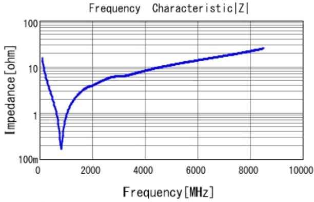
GRM1555C2A101GA01 |Z| DCOV, 25degC
