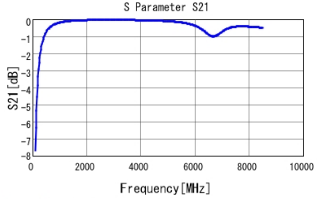
GRM1555C1H7R2DA01 S21 DCOV, 25degC
