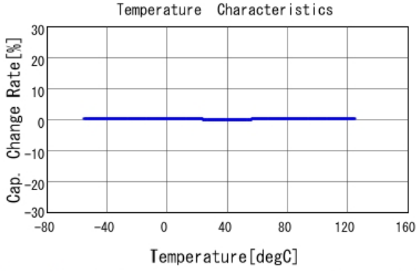
GRM1555C1H7R2DA01 C-Temp. capchange, DCOV, AC1Vrms
