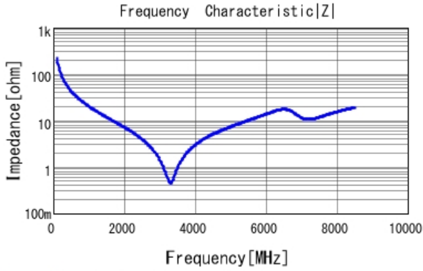
GRM1555C1H7R2DA01 |Z| DCOV, 25degC
