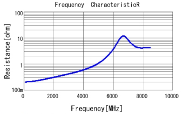
GRM1555C1H7R2DA01 R DCOV, 25degC
