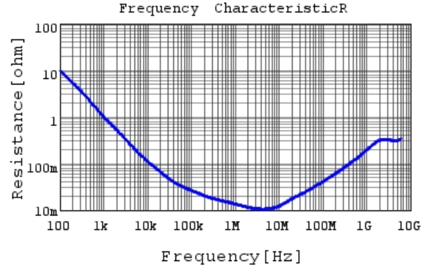
GRM033R60J225ME47 R DC0V, 25degC
