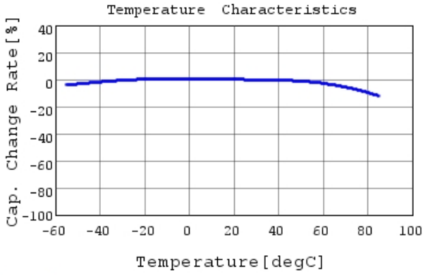
GRM033R60J225ME47 C-Temp. capchange, DC0.0V,
