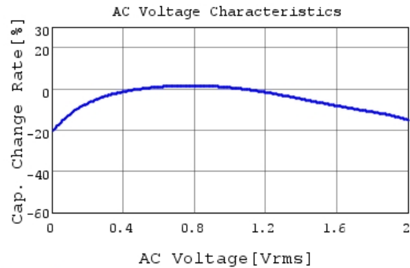
GRM033R60J225ME47 C-AC Voltage capchange, DC
