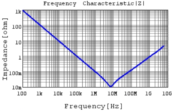
GRM033R60J225ME47 |Z| DC0V, 25degC
