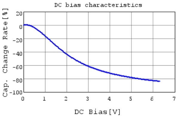
GRM033R60J225ME47 C-DC bias capchange, 25.0c
