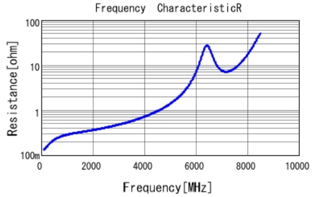
GRM1885C2A5R0CA01 R DCOV, 25degC
