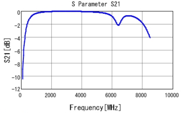
GRM1885C2A5R0CA01 S21 DCOV, 25degC
