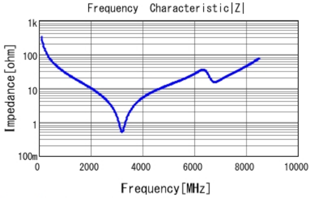
GRM1885C2A5R0CA01 |Z| DCOV, 25degC
