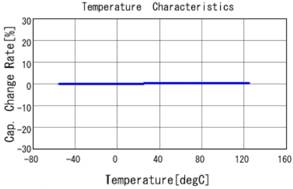
GRM1885C2A5R0CA01 C-Temp. capchange, DCOV, AC1Vrms
