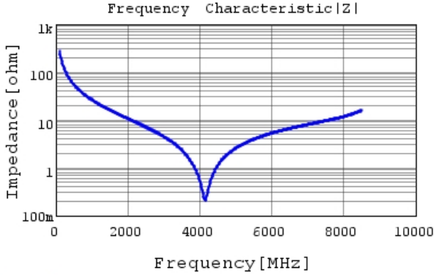
GJM0335C1E5R7DB01 |Z| DC0V, 25degC
