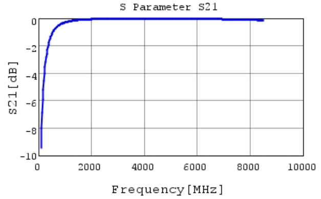
GJM0335C1E5R7DB01 S21 DCOV, 25degC
