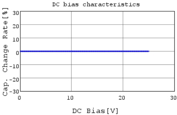
GJM0335C1E5R7DB01 C-DC bias capchange, 25.0c
