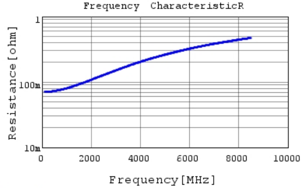
GJM0335C1E5R7DB01 R DC0V, 25degC
