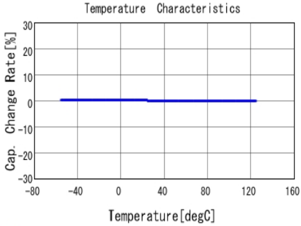
■ GCM1885C2A220JA16 C-Temp. capchange, DCOV, AC1Vrms
