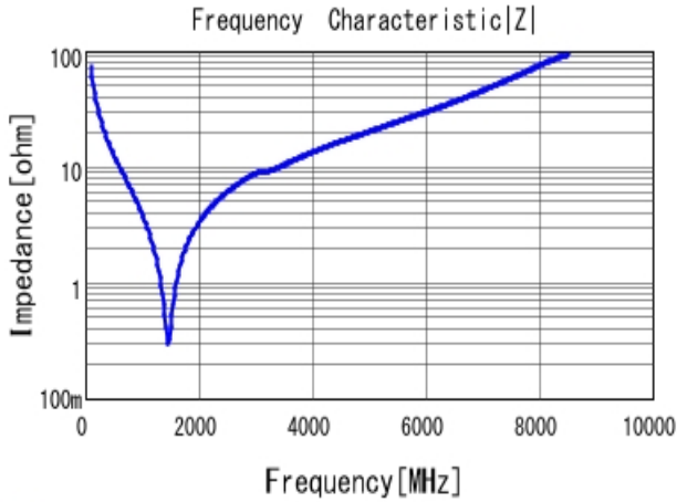
■ GCM1885C2A220JA16 |Z| DC0V, 25degC
