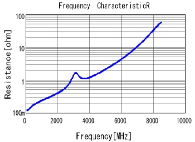
■ GCM1885C2A220JA16 R DC0V, 25degC
