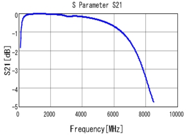
■ GCM1885C2A220JA16 S21 DCOV, 25degC
