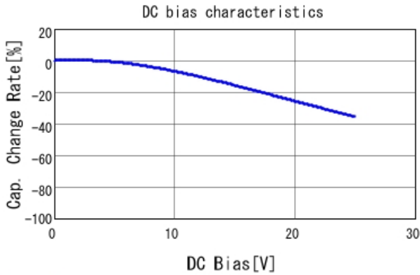
GRM219R71E224MA01 C-DC bias capchange, 25.0degC, A
