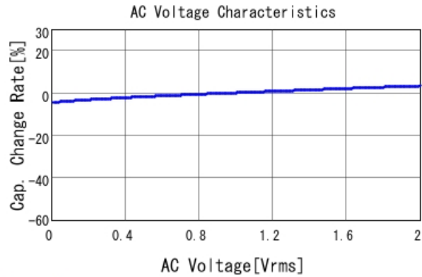
GRM219R71E224MA01 C-AC Voltage capchange, DCOV, 25
