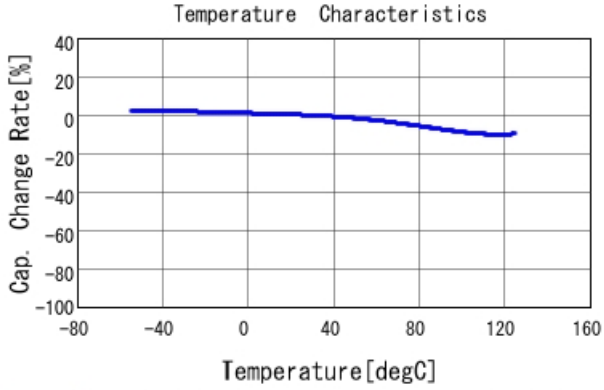
GRM219R71E224MA01 C-Temp. capchange, DC0.0V, AC1.C
