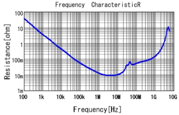
GRM219R71E224MA01 R DCOV, 25degC
