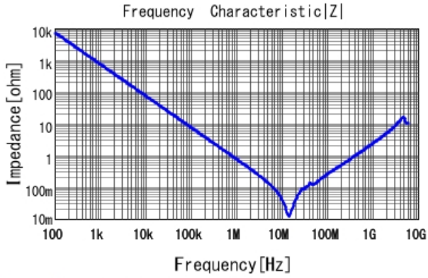
GRM219R71E224MA01 |Z| DCOV, 25degC
