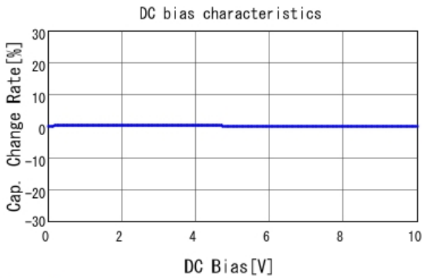
GRM21B7U1A104JA01 C-DC bias capchange, 25.0degC, A
