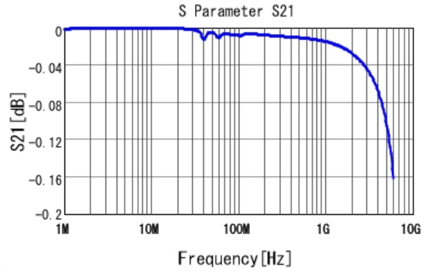
GRM21B7U1A104JA01 S21 DCOV, 25degC
