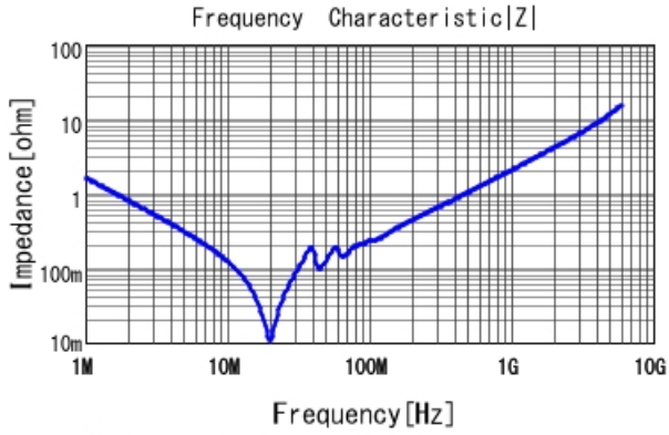
GRM21B7U1A104JA01 |Z| DCOV, 25degC
