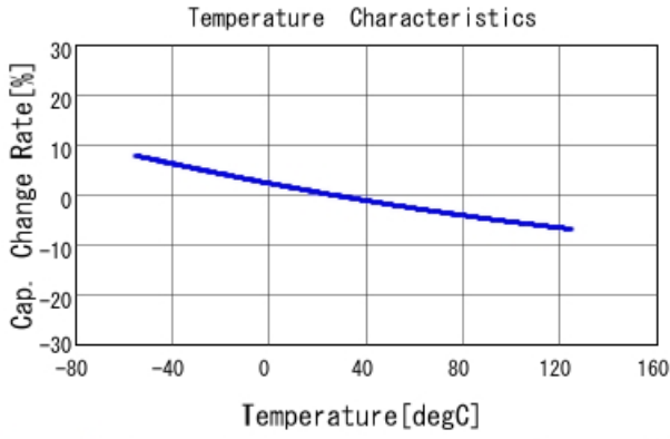
GRM21B7U1A104JA01 C-Temp. capchange, DCOV, AC1Vrms
