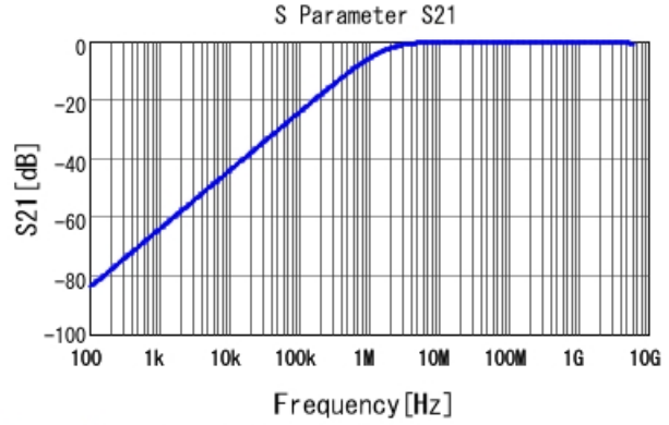
GRM188R72A102KA01 S21 DC0V, 25degC
