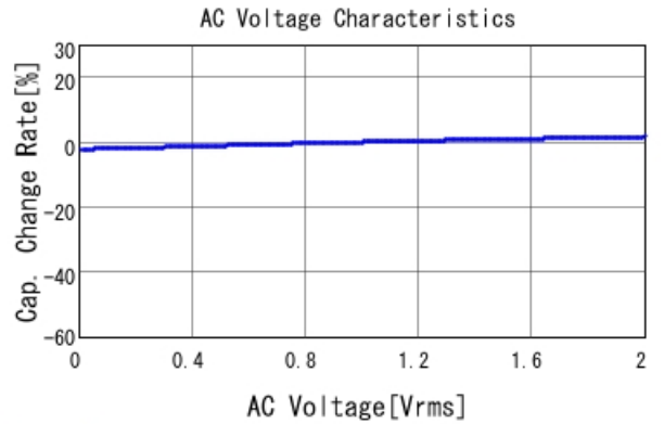
GRM188R72A102KA01 C-AC Voltage capchange, DCOV, 25
