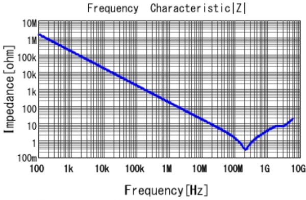
GRM188R72A102KA01 |Z| DCOV, 25degC
