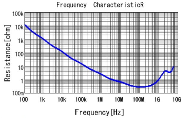
GRM188R72A102KA01 R DCOV, 25degC
