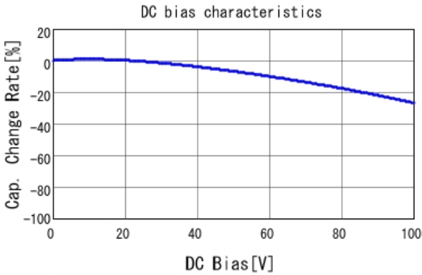
GRM188R72A102KA01 C-DC bias capchange, 25.0degC, A
