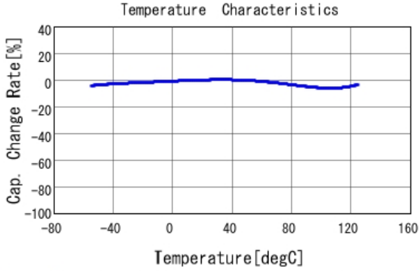
GRM188R72A102KA01 C-Temp. capchange, DC0.0V, AC1.C
