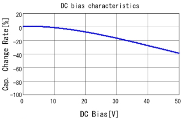
GRM188R61H223KA01 C-DC bias capchange, 25.0degC, A
