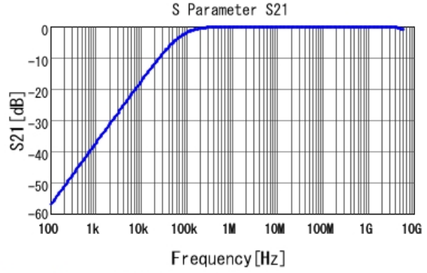
GRM188R61H223KA01 S21 DC0V, 25degC
