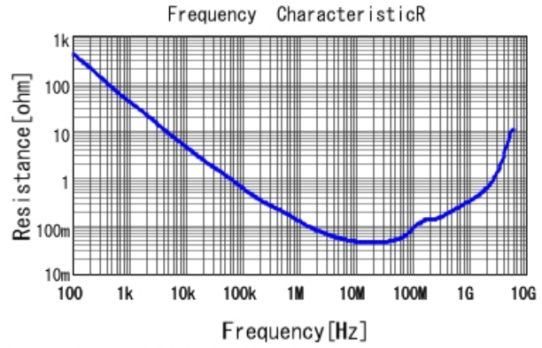
GRM188R61H223KA01 R DCOV, 25degC
