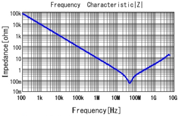
GRM188R61H223KA01 |Z| DCOV, 25degC
