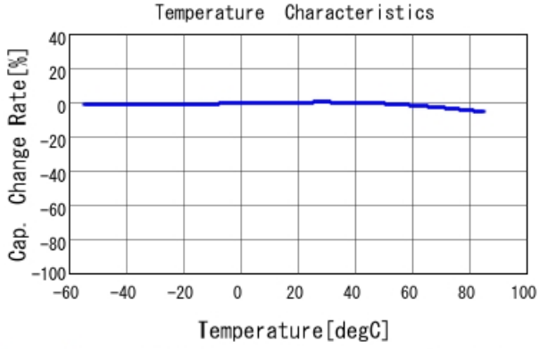
GRM188R61H223KA01 C-Temp. capchange, DC0.0V, AC1.C
