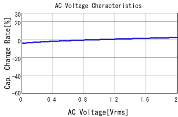
GRM188R61H223KA01 C-AC Voltage capchange, DCOV, 25
