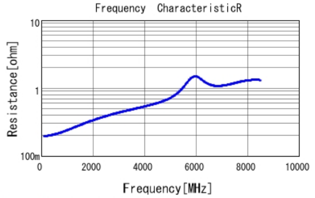
GRM1555C2A8R5CA01 R DCOV, 25degC
