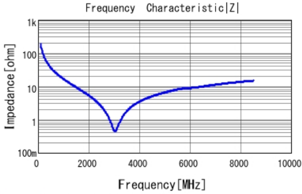
GRM1555C2A8R5CA01 |Z| DCOV, 25degC
