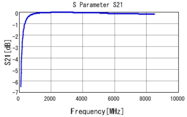
GRM1555C2A8R5CA01 S21 DCOV, 25degC
