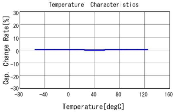
GRM1555C2A8R5CA01 C-Temp. capchange, DCOV, AC1Vrms
