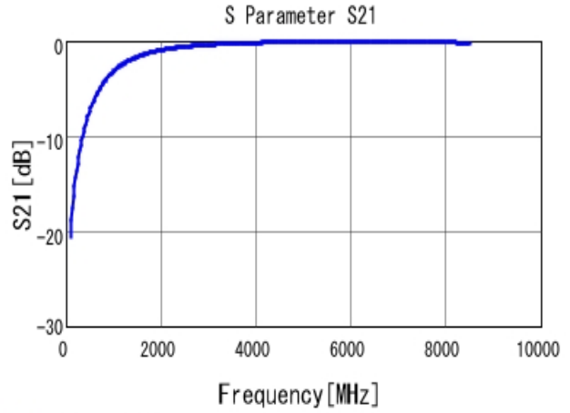
■ GRM1554C1H1R5CA01 S21 DCOV, 20degC
