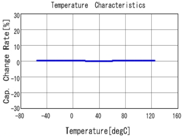
■ GRM1554C1H1R5CA01 C-Temp. capchange, DCOV, AC1Vrms
