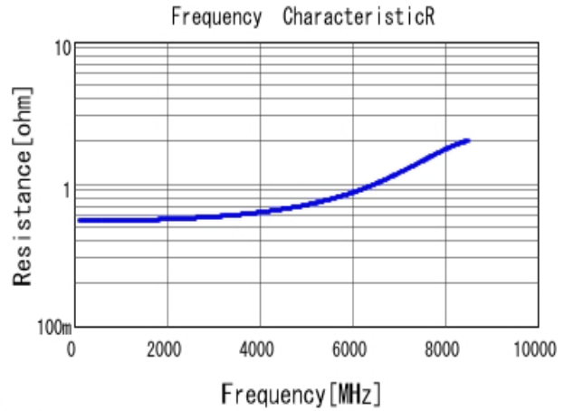
■ GRM1554C1H1R5CA01 R DCOV, 20degC
