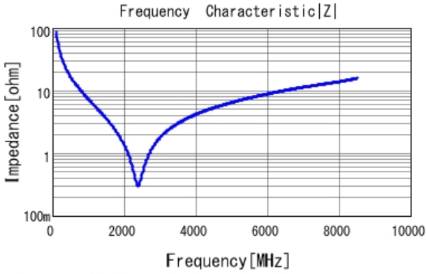
■ GRT0335C1H180JA02 |Z| DC0V, 25degC
