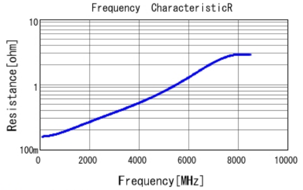
■ GRT0335C1H180JA02 R DC0V, 25degC
