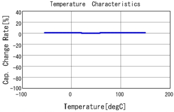
GCM1555G1H561JA16 C-Temp. capchange, DCOV, AC1Vrms
