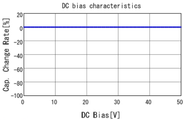
GCM1555G1H561JA16 C-DC bias capchange, 25.0degC, A
