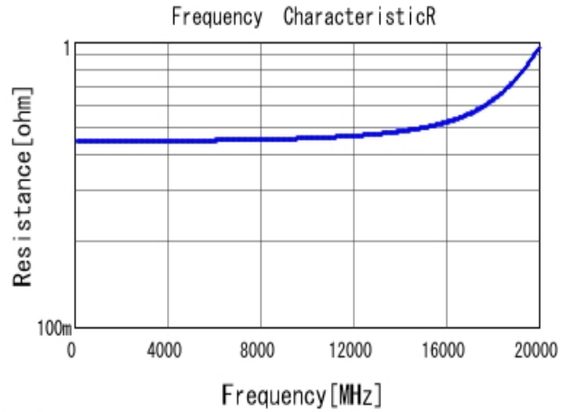
■ GJM0335C1HR50BB01 R DC0V, 25degC
