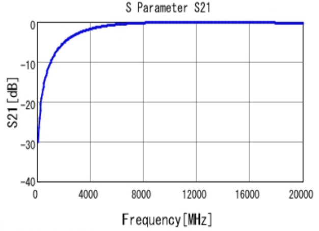
■ GJM0335C1HR50BB01 S21 DCOV, 25degC
