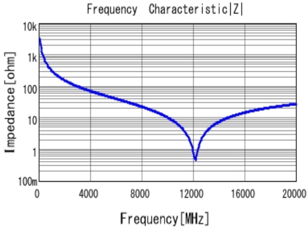
■ GJM0335C1HR50BB01 |Z| DC0V, 25degC
