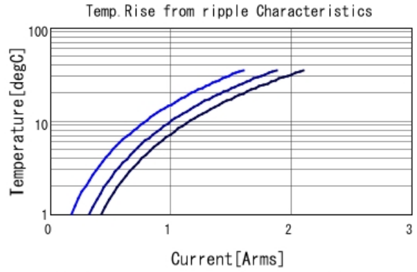
GRM188R71H154MAC4 Temp. rise — 400kHz — 800I
