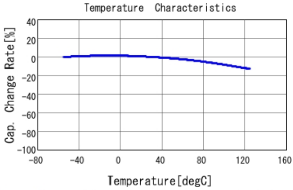
GRM188R71H154MAC4 C-Temp. capchange, DC0.0V, AC1.C
