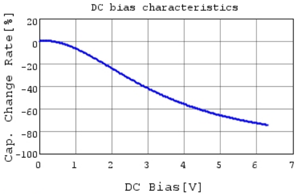
GRM31CD80J107MEA8 C-DC bias capchange, 25.0c
