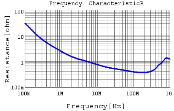
RCER73A102K2K1H03B R DCOV, 25degC
