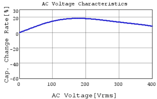
RCER73A102K2K1H03B C-AC Voltage capchange, I
