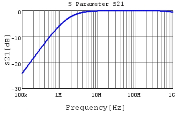
RCER73A102K2K1H03B S21 DCOV, 25degC
