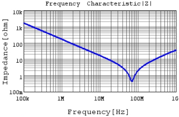
RCER73A102K2K1H03B |Z| DCOV, 25degC
