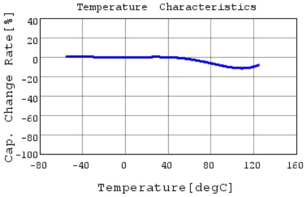
RCER73A102K2K1H03B C-Temp. capchange, DCOV,
