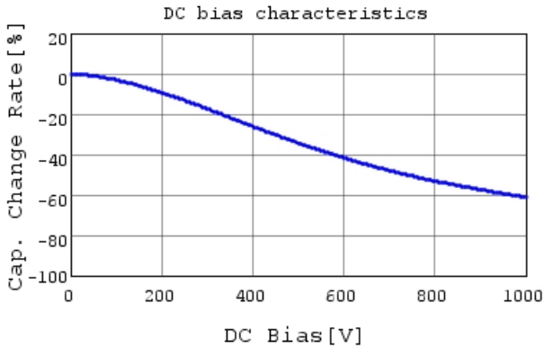
RCER73A102K2K1H03B C-DC bias capchange, 25.0
