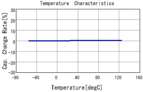
GRM1885C1H5R2BA01 C-Temp. capchange, DC0V, AC1Vrms
