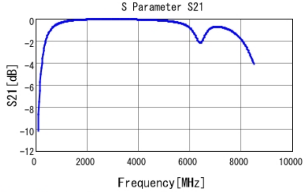
GRM1885C1H5R2BA01 S21 DC0V, 25degC
