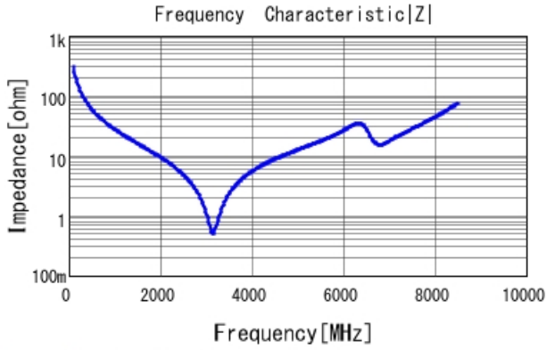
GRM1885C1H5R2BA01 |Z| DCOV, 25degC
