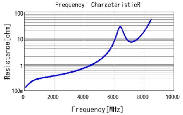
GRM1885C1H5R2BA01 R DCOV, 25degC
