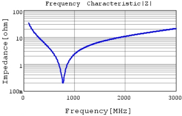
GRM31A5C2J470JW01 |Z| DC0V, 25degC
