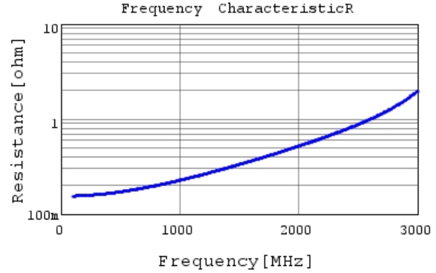
GRM31A5C2J470JW01 R DC0V, 25degC
