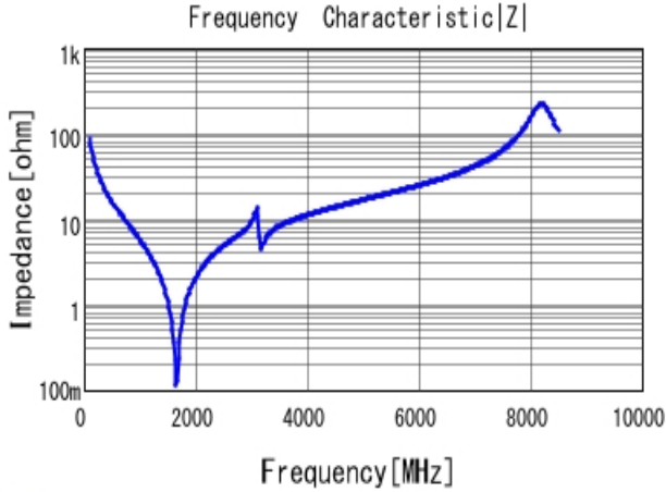
■ GQM1885C1H180JB01 |Z| DCOV, 25degC
