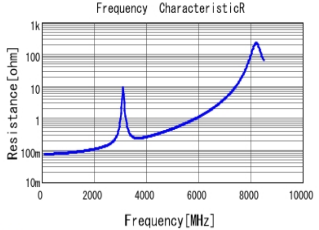
■ GQM1885C1H180JB01 R DCOV, 25degC
