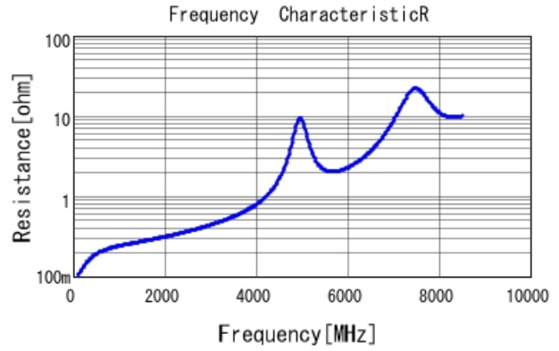
GRM1885C2A9R3DA01 R DCOV, 25degC
