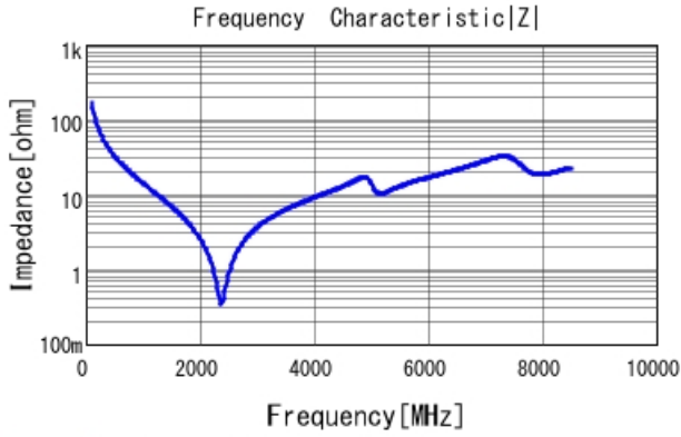
GRM1885C2A9R3DA01 |Z| DCOV, 25degC
