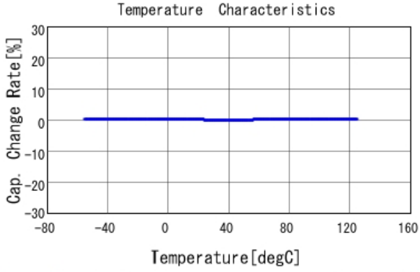
GRM1555C1H8R2CA01 C-Temp. capchange, DCOV, AC1Vrms
