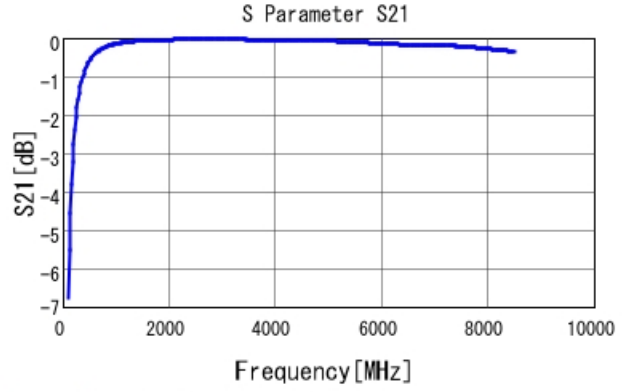
GRM1555C1H8R2CA01 S21 DCOV, 25degC
