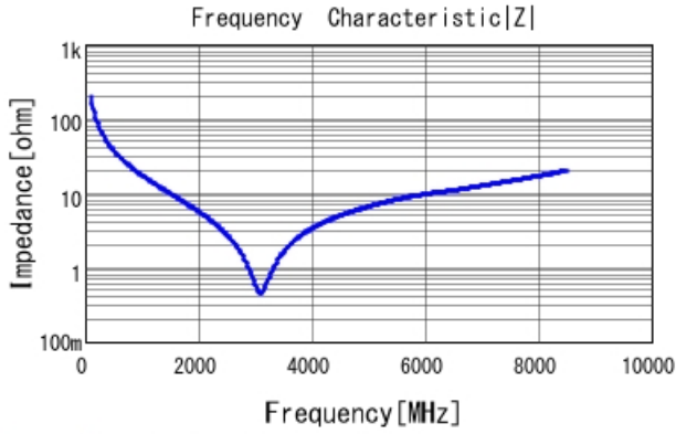
GRM1555C1H8R2CA01 |Z| DCOV, 25degC
