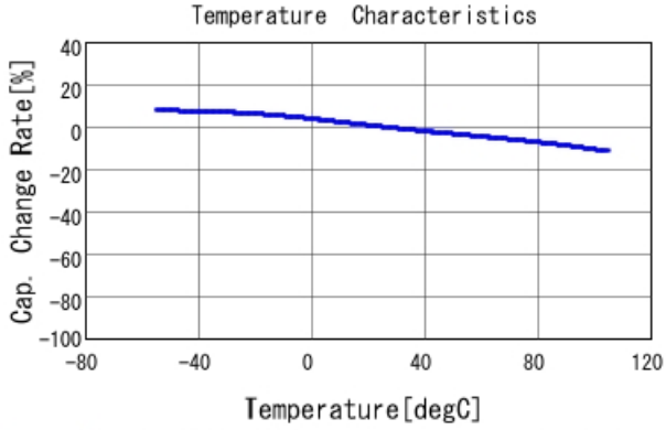
GRM155C81H104KE19 C-Temp. capchange, DC0.0V, AC1.C
