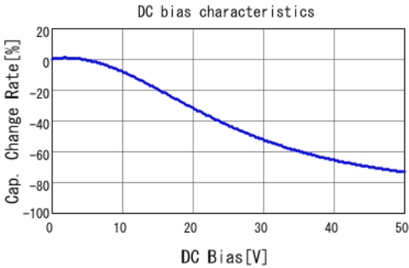
GRM155C81H104KE19 C-DC bias capchange, 25.0degC, A
