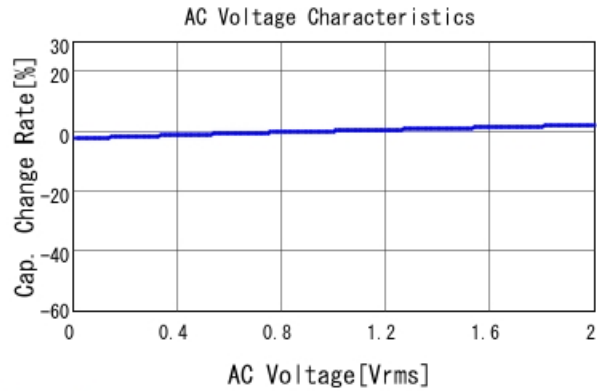
GRM155C81H104KE19 C-AC Voltage capchange, DCOV, 25
