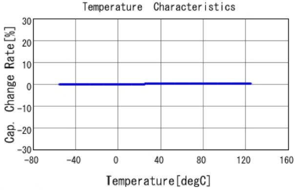
GJM0335C1E5R4WB01 C-Temp. capchange, DC0V, AC1Vrms
