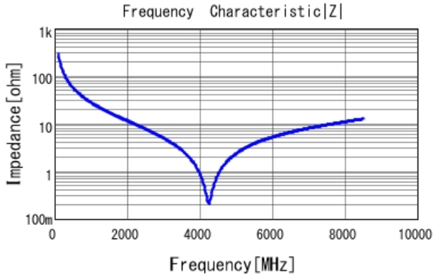
GJM0335C1E5R4WB01 |Z| DC0V, 25degC
