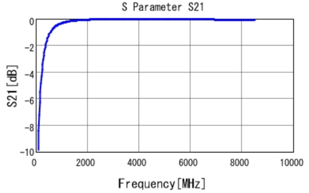
GJM0335C1E5R4WB01 S21 DC0V, 25degC
