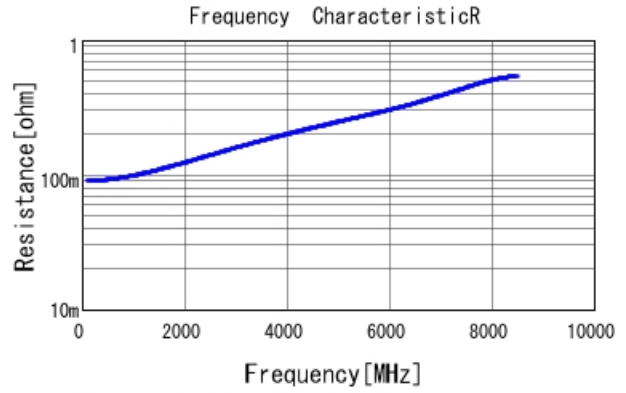
GJM0335C1E5R4WB01 R DC0V, 25degC
