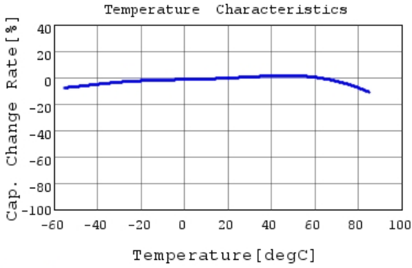
GRM155R60J475ME47 C-Temp. capchange, DC0.0V,
