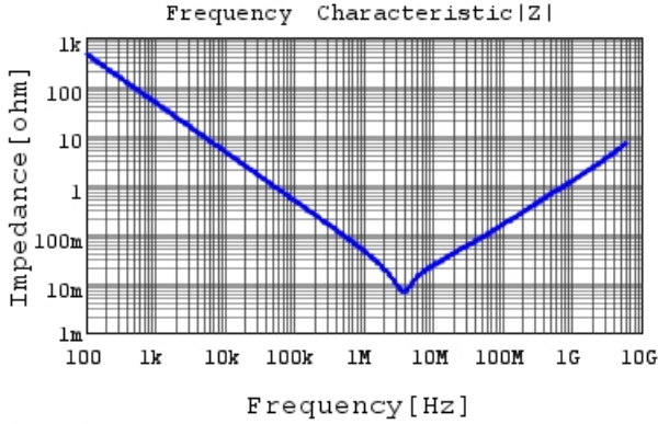
GRM155R60J475ME47 |Z| DC0V, 25degC
