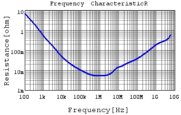
GRM155R60J475ME47 R DC0V, 25degC
