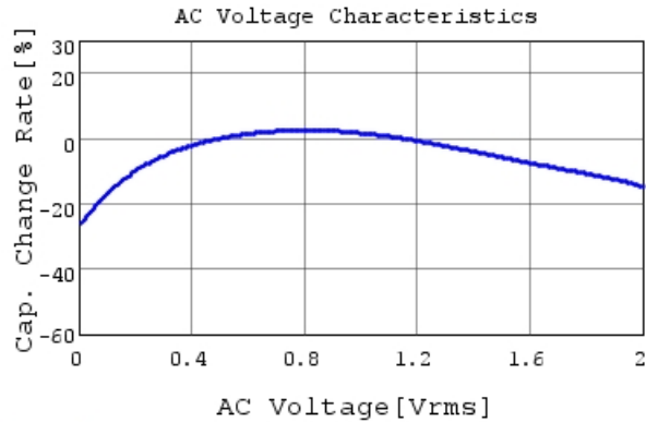
GRM155R60J475ME47 C-AC Voltage capchange, DC
