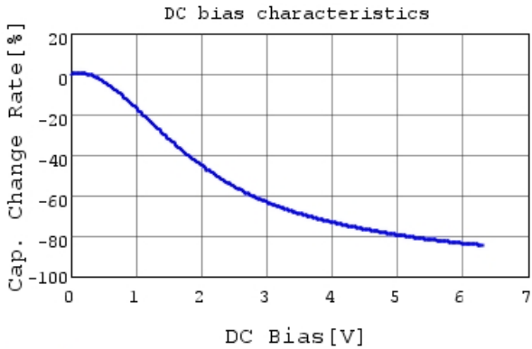
GRM155R60J475ME47 C-DC bias capchange, 25.0c
