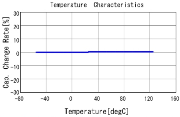
GRM1885C1H5R2WA01 C-Temp. capchange, DC0V, AC1Vrms
