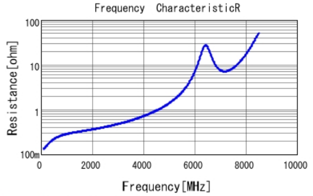
GRM1885C1H5R2WA01 R DCOV, 25degC
