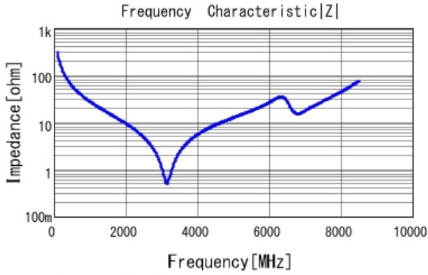
GRM1885C1H5R2WA01 |Z| DCOV, 25degC
