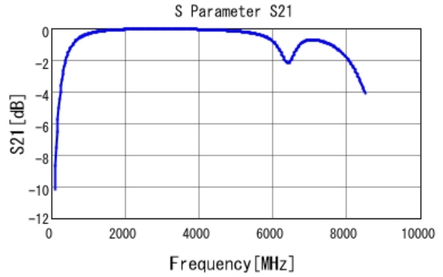
GRM1885C1H5R2WA01 S21 DC0V, 25degC
