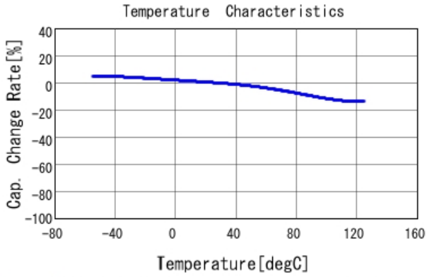
GRT155R71C223KE01 C-Temp. capchange, DC0.0V, AC1.C
