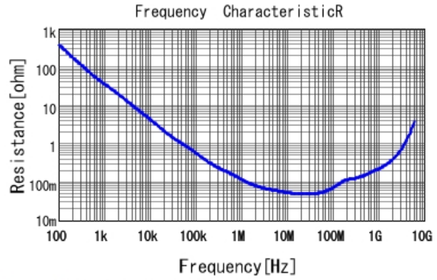
GRT155R71C223KE01 R DCOV, 25degC
