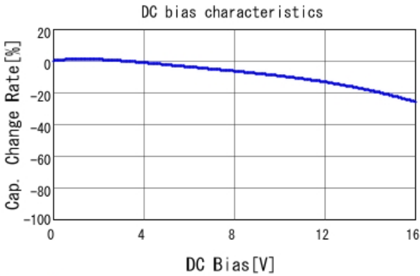
GRT155R71C223KE01 C-DC bias capchange, 25.0degC, A
