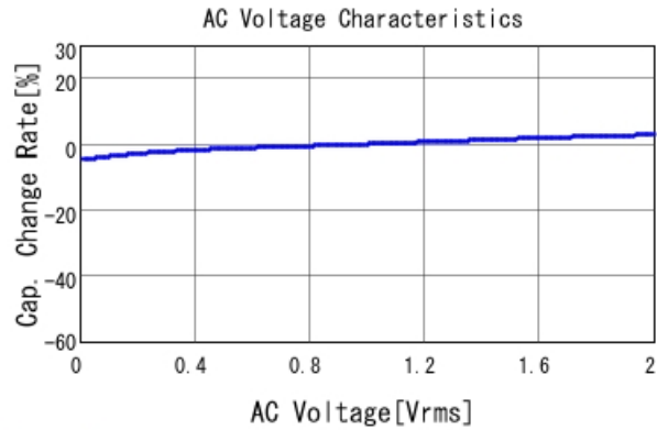
GRT155R71C223KE01 C-AC Voltage capchange, DCOV, 25
