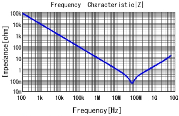
GRT155R71C223KE01 |Z| DCOV, 25degC
