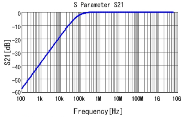
GRT155R71C223KE01 S21 DC0V, 25degC
