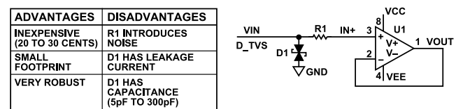
Figure 65. ESD Protection Circuit (R-TVS Network)
