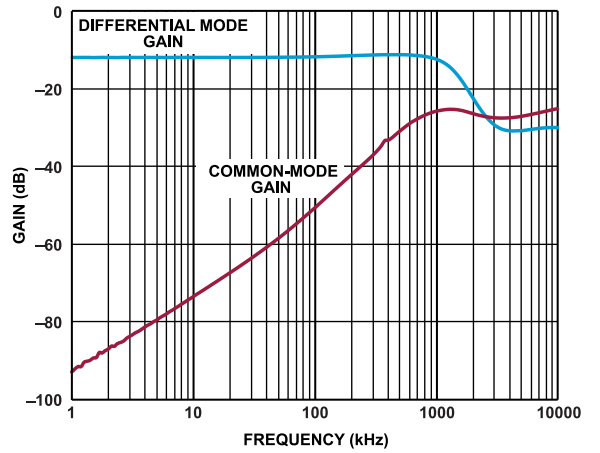
Figure 68. \pm 10\text{ V} to 0\text{ V} to +5\text{ V} Funnel Amplifier, System Gain
