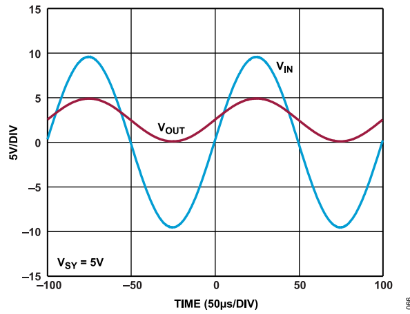
Figure 67. \pm 10\text{ V} to 0\text{ V} to +5\text{ V} Funnel Amplifier, Input and Output Voltages
