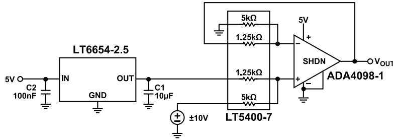
Figure 66. \pm 10\text{ V} to 0\text{ V} to +5\text{ V} Funnel Amplifier, High CMRR and \pm 80\text{ V} Input Protection via LT5400-7 Resistor Network (ADA4098-1 6-Lead TSOT)
